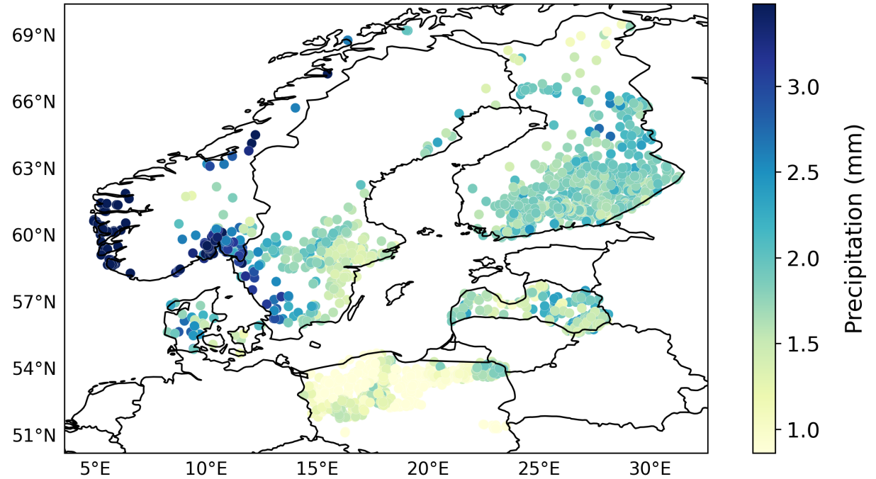
Daily mean precipitation
