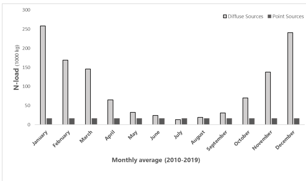
Figure 11. Monthly nitrogen supply to Odense Fjord, distributed between diffuse sources and point sources. Average for the years 2010-2019. Data from Aarhus University.
