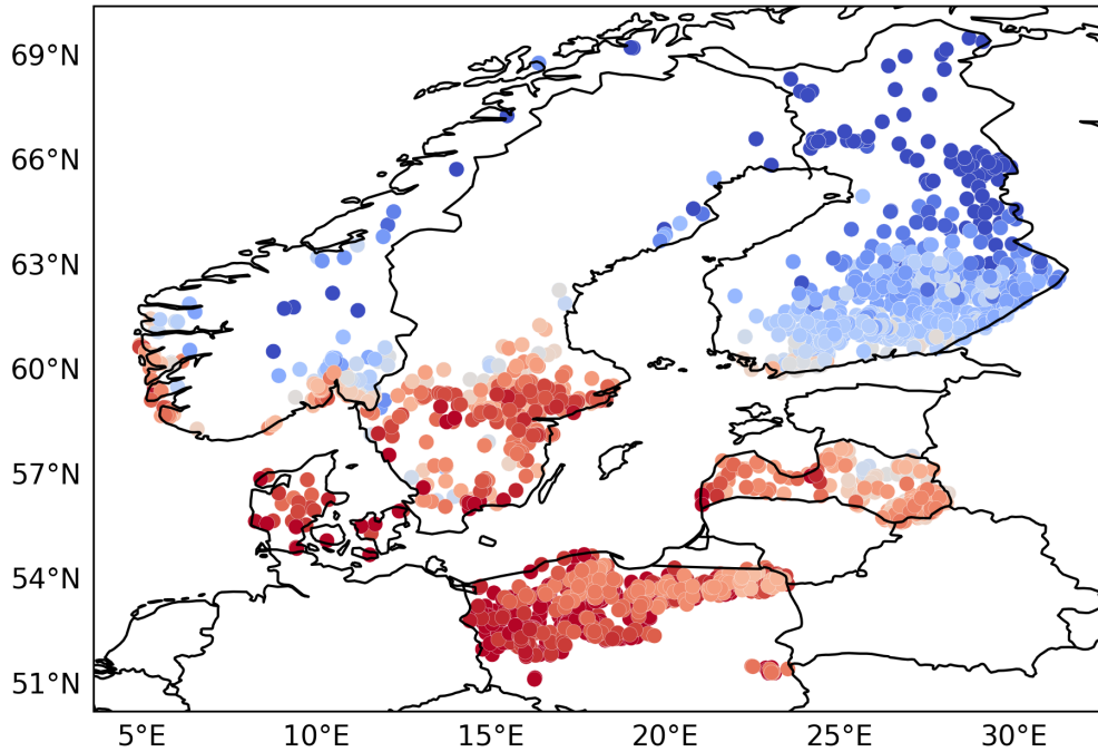
Annual mean air temperature
