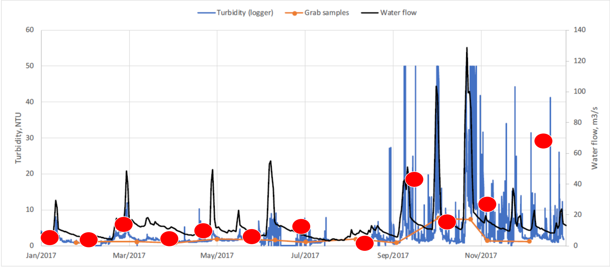
Figure 52. Turbidity and water flow at the outlet of Storelva in 2017. The water flow data are from NVE.
