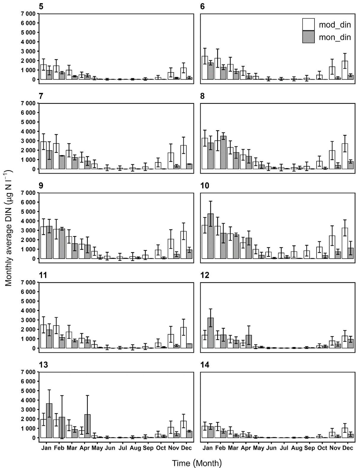
Figure 13. Odense Fjord, Denmark. Simulated and measured concentrations of DIN in Odense Inner Fjord as defined by the WFD. Notice that modelled data are from 2002-2026 whereas monitored data are from June 2002-2023.
