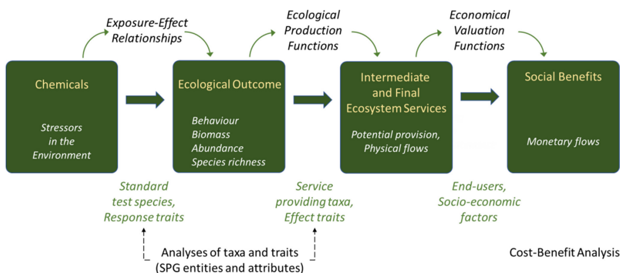
Figure 27. The translation of effect data from standardised ecotoxicological testing for ES impact assessment using ecotoxicological exposure-effect relationships and ecological production functions based on response traits and functional traits (also called ‘effect traits’) respectively. EPFs quantify potential provision of intermediate or final services, and socio-economic factors determine actual flows of services ‘physical flows’ and benefits ‘monetary flows’.
