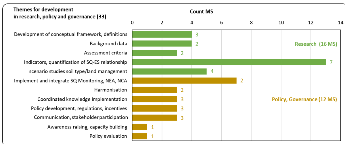
Figure 20. Knowledge gaps indicated by the Member States in relation to implementation of SQ-based ES assessment, categorised under general themes for development in research (green bars) or policy and governance (brown bars). The diversity of specific needs is indicated per theme at the top of the bars (specified in Table D7). Research needs were specified by 16 MS, and 12 MS indicated policy development needs; a total of 50 specifications were received over 33 different gaps.
