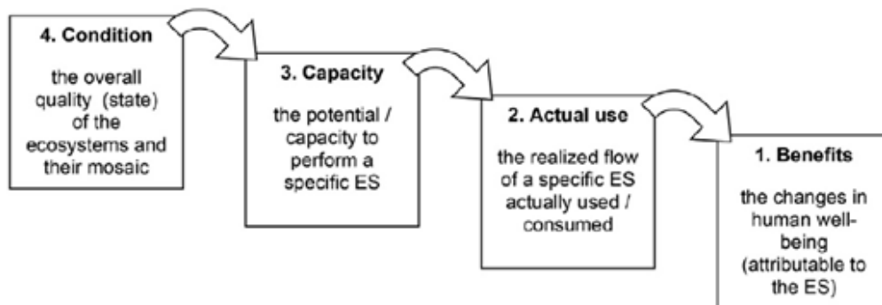
Figure 26. The cascade model (Czucz et al. 2020).
