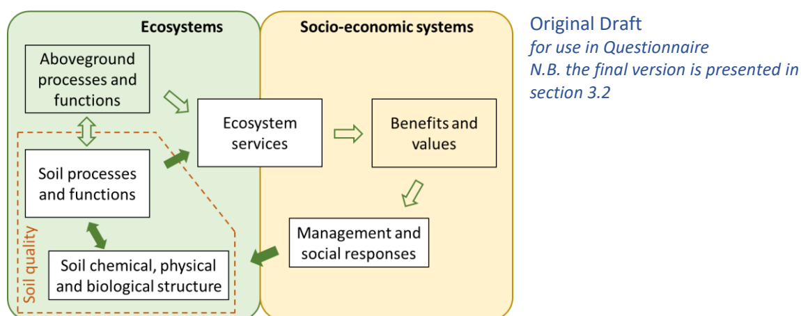
Figure 2. Integrating the relationship between ecological (left, green) and socio-economic (right, yellow) systems for agricultural soils will provide a more comprehensive approach for evaluation and decision-making in policy and management (Adapted from Liqueste et al. 2016). Highlighted boxes (white) and filled arrows (green) represent the focus of the SIREN study. Note: This scheme was drafted at the start of the project, and has been elaborated to more detail towards the end; a final version is presented in Chapter 3 Synthesis.
