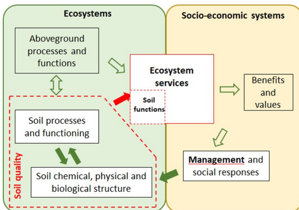
Figure 11. Draft framework linking soil quality to ecosystem services.
