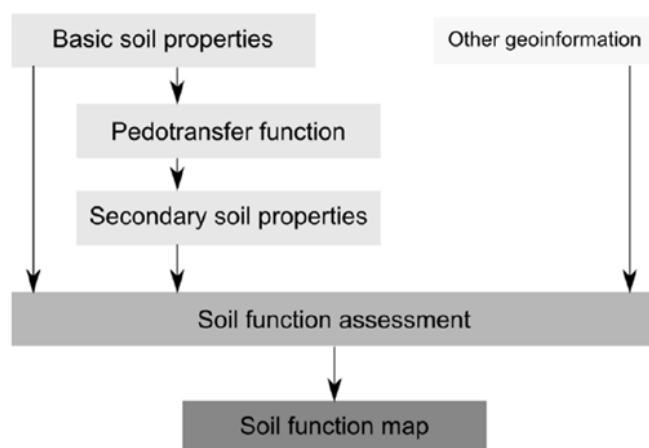
Figure 25. The soil function assessment workflow (Greiner et al. 2017).
