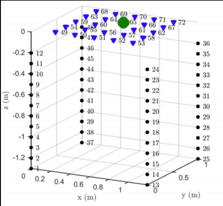
Small scale characterization of vine plant root water uptake via 3D electrical resistivity tomography . Benjamin Mary 2018; Myrian S.
